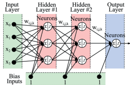
Fig. 7. Architecture of Recurrent Neural Network
